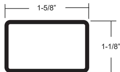
Top Rail Profile
