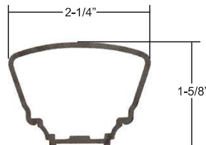
Top Rail Profile
