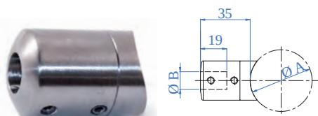
Tondo - Round
