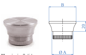
Massicci - Solid
