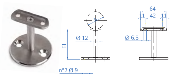
Reggicorrimano flangiato Flanged handrail support
