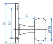
Door knob with shield right / left handed
